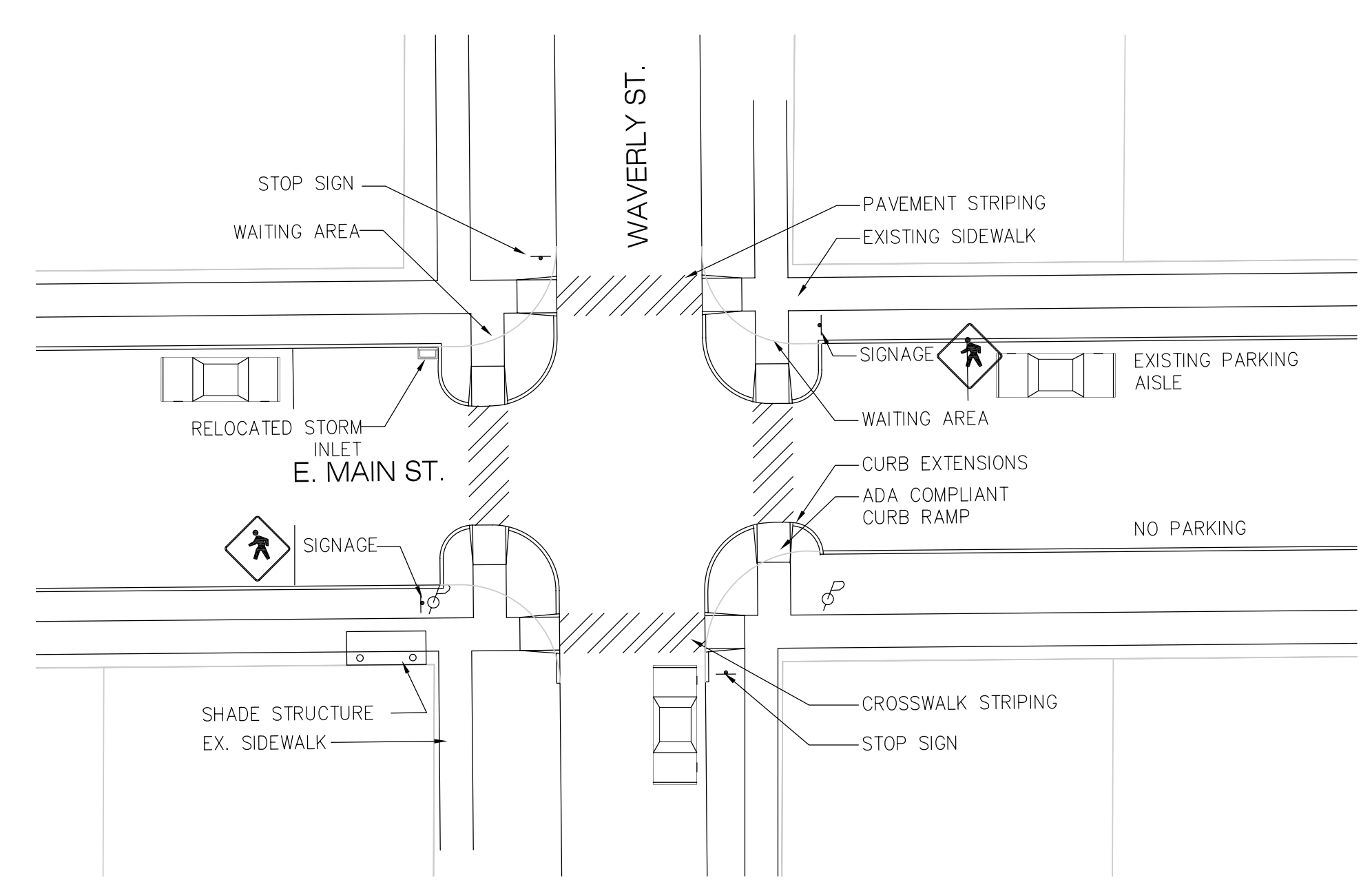
INTERSECTION OF E. MAIN ST. & WAVERLY ST. NOT TO SCALE
