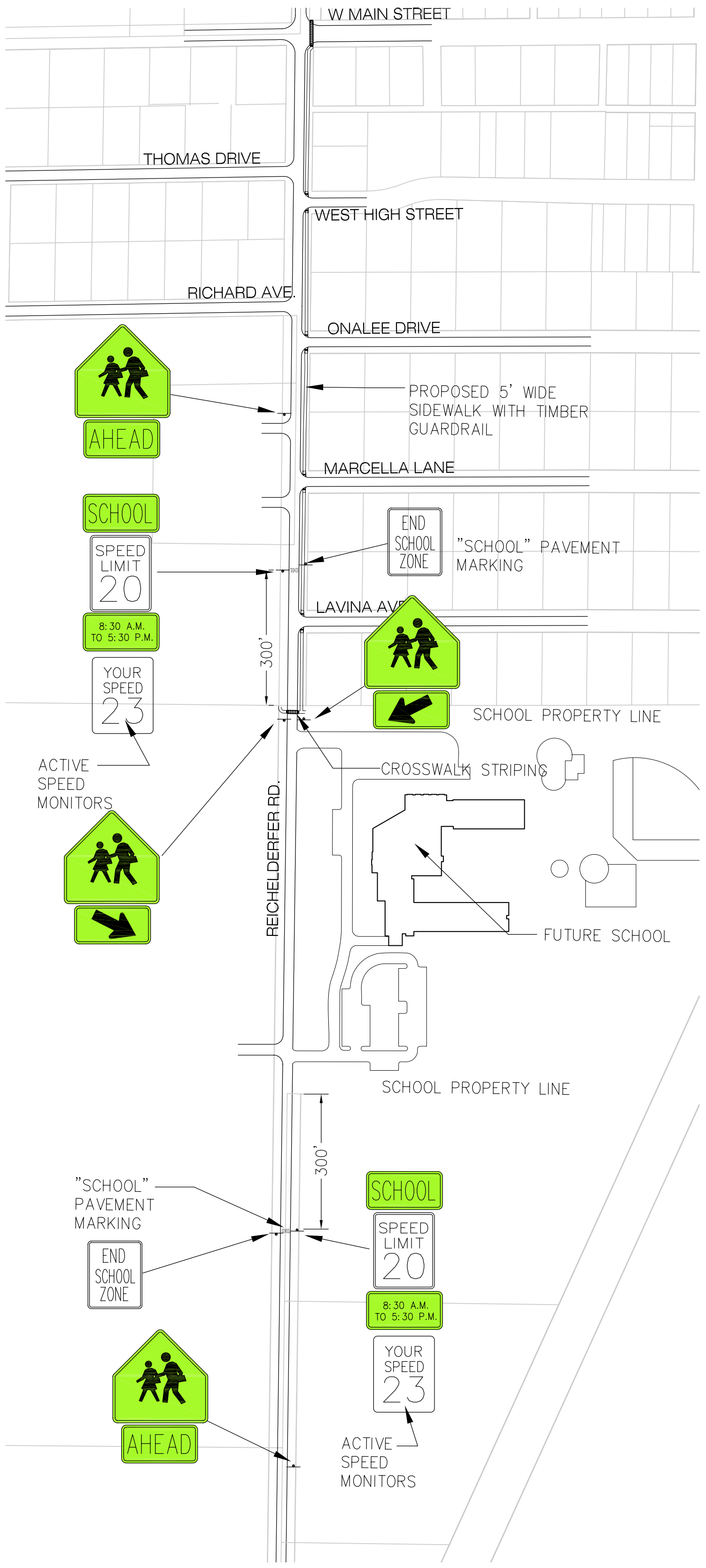
SCHOOL AREA TRAFFIC CONTROL MEASURES NOT TO SCALE
