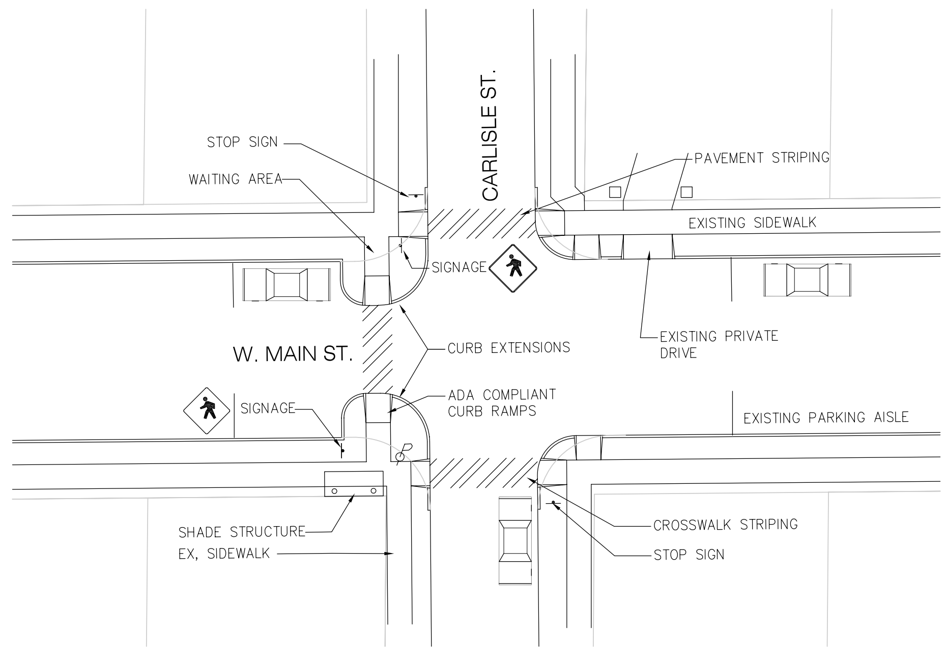
INTERSECTION OF W. MAIN ST. & CARLISLE ST. NOT TO SCALE
